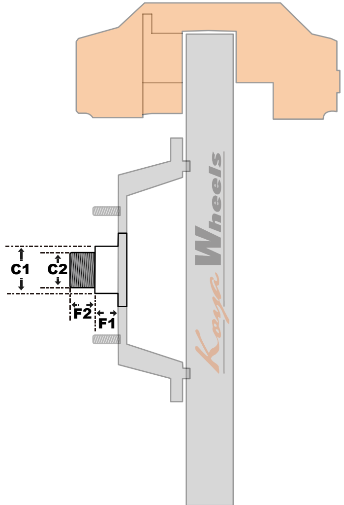
Hub & Axle 2D Side View
