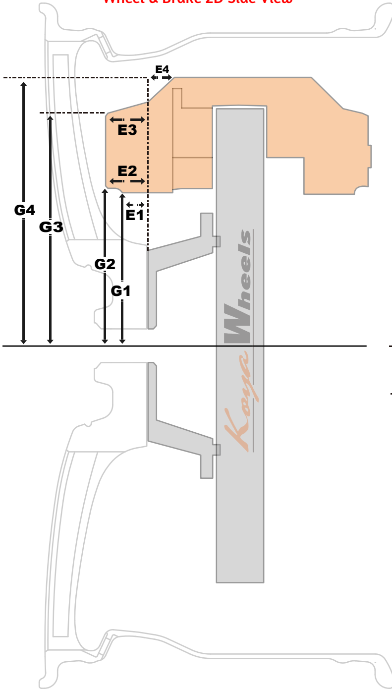
Wheel & Brake 2D Side View
